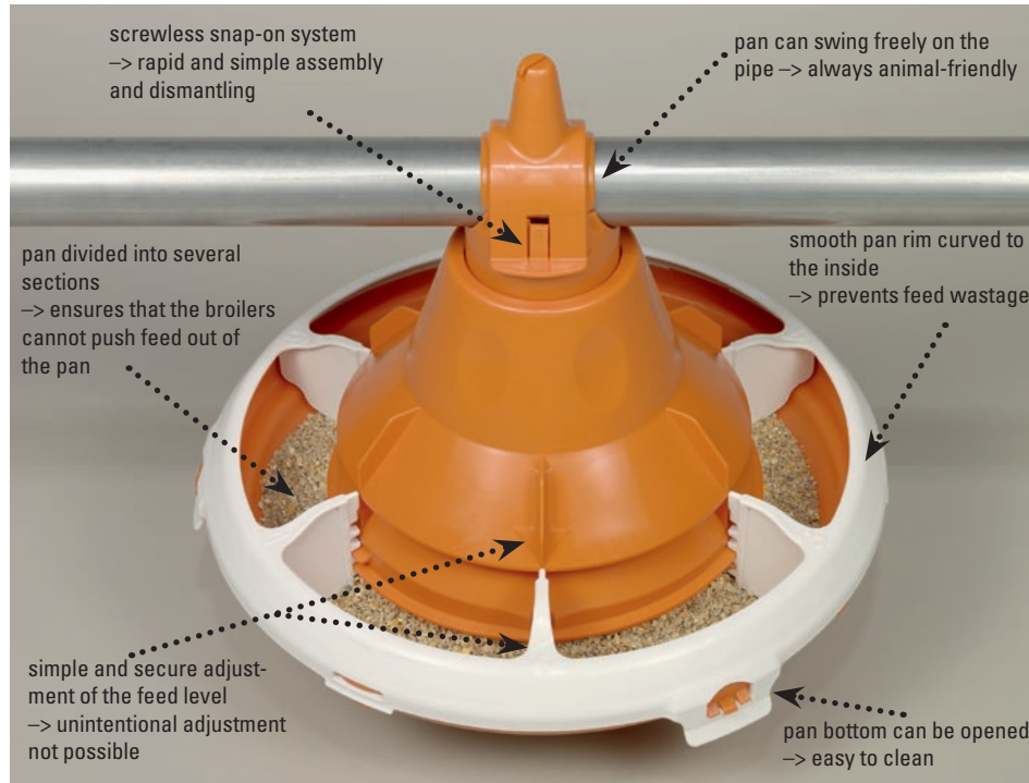
Vista 360 – chicks can easily access the feed in the pan
